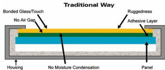
Optical Bonding
