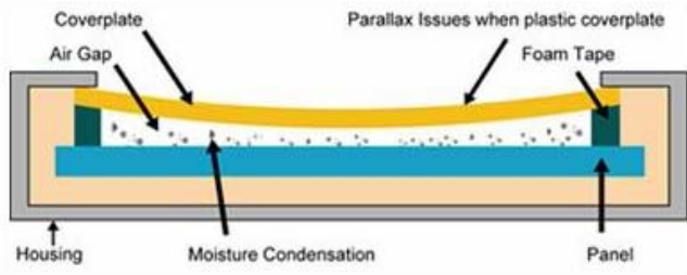
Traditional way: Use Foam tape to fix the glass ==> Air Gap
